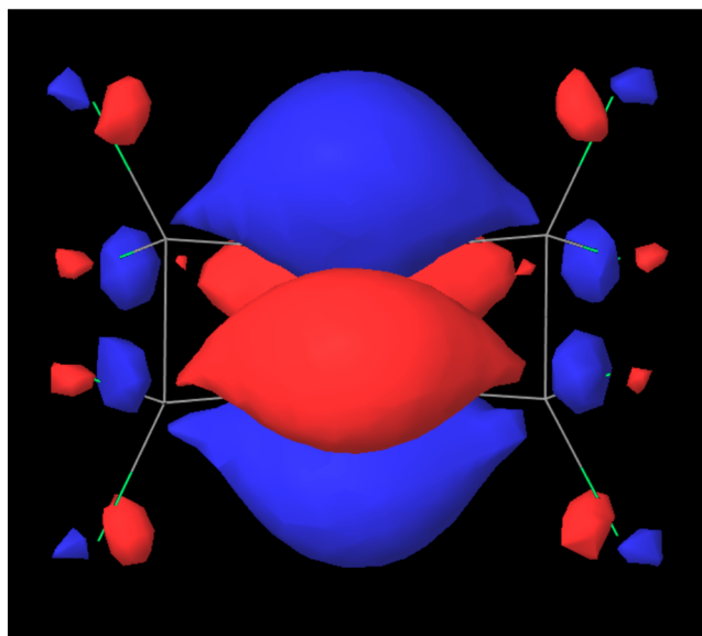
Figure 4. LUMO of alkene 1 (B3LYP/6-311G**+ level of theory). 19
